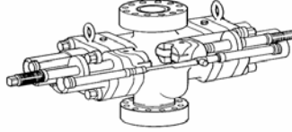
Cameron Dual Flex Bore Rams
