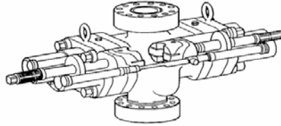
Hydril Dual Bore Rams
