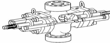
Hydril Variable Bore Rams
